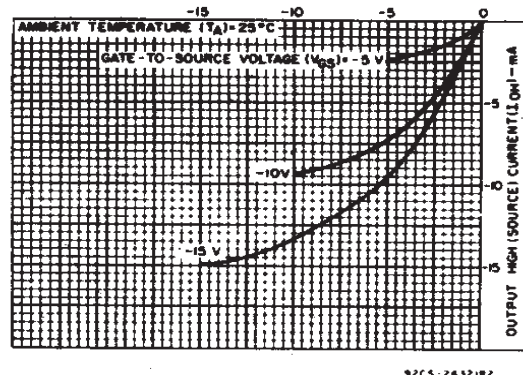
Figure 8. Minimum Output High (Source) Current Characteristics
